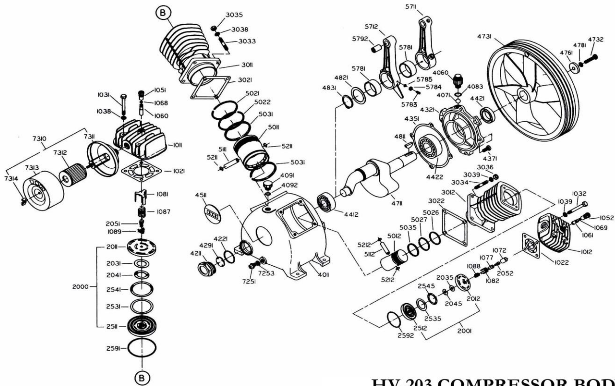
HV-203 COMPRESSOR BODY
