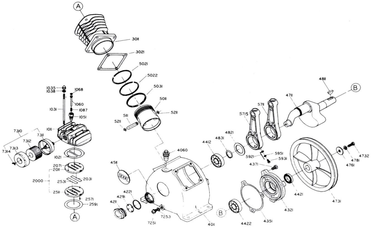
SV-202 COMPRESSOR BODY
